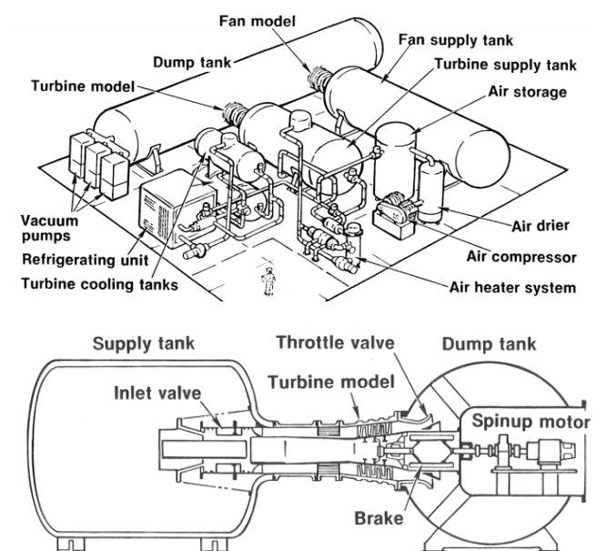
Figure 3. Proposed turbine/fan test facility at UTRC, Case [1985] (not constructed)
