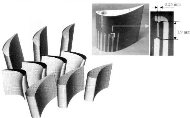
Figure 13. 1 ½ stage VKI turbine research rig operational conditions, Sieverding et al. [1992,1998], and two-layered “Senflex” thin film heat transfer gauge array attached on the suction side of the second stator, Illiopoulou et al. [2004]
