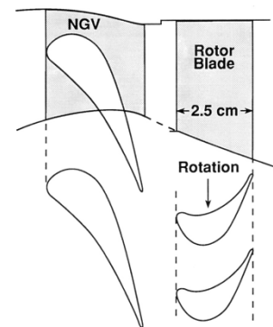
Fig. 1: Transonic turbine geometry investigated
