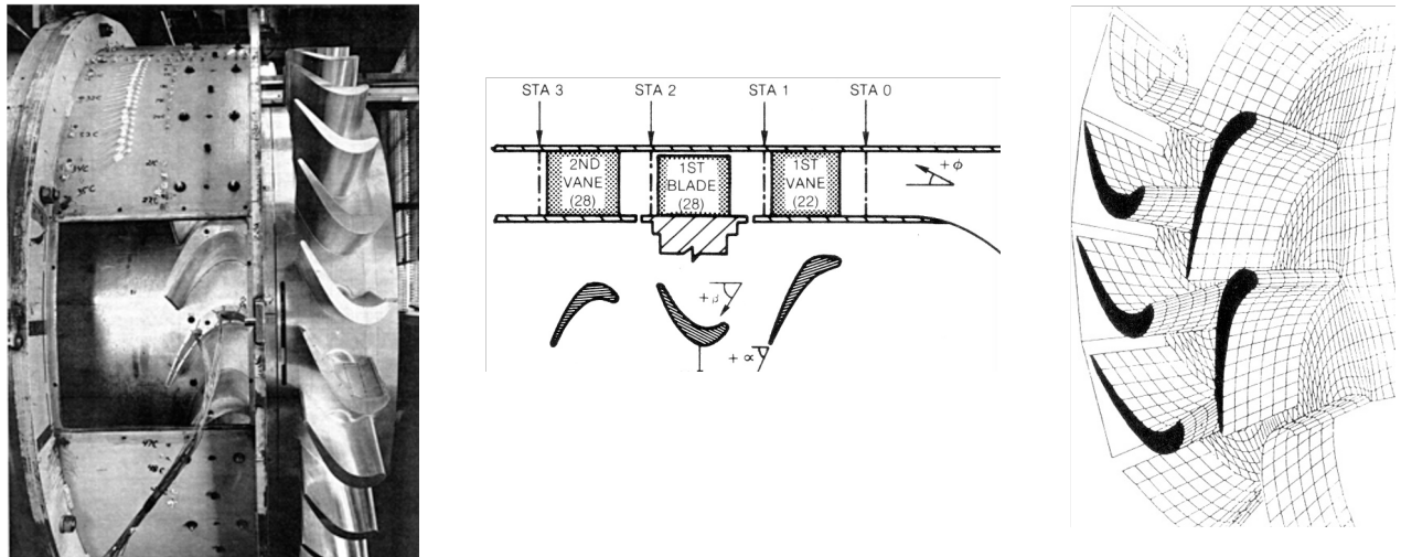
Figure 7. UTRC's Large Scale Rotating Rig (LSRR), Dring and Joslyn [1981]
