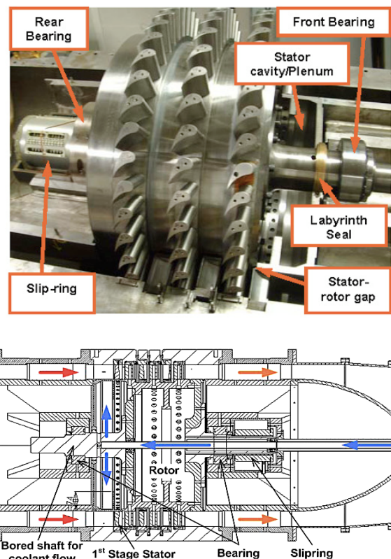
Figure 19 Three-stage, low-speed large-scale turbine facility at Texas A&M University Schoebei et al. [2000]
