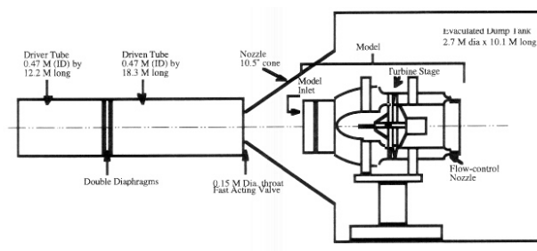
Figure 16. Shock tube driven turbine test facility at the Ohio State University, Dunn and Haldeman (2000)
