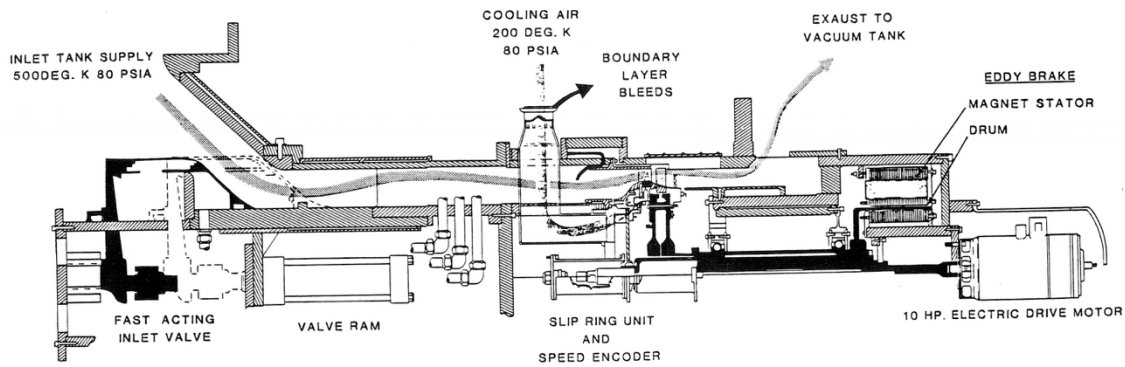
Figure 5. MIT turbine test section and fast-acting inlet valve, Epstein et al. [1984]
