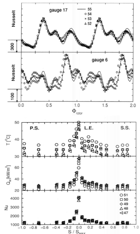
Figure 14. Phase-locked unsteady heat transfer measurements and time-averaged heat transfer on the second stator of the VKI turbine research facility, Illiopoulou et. al (2004)
