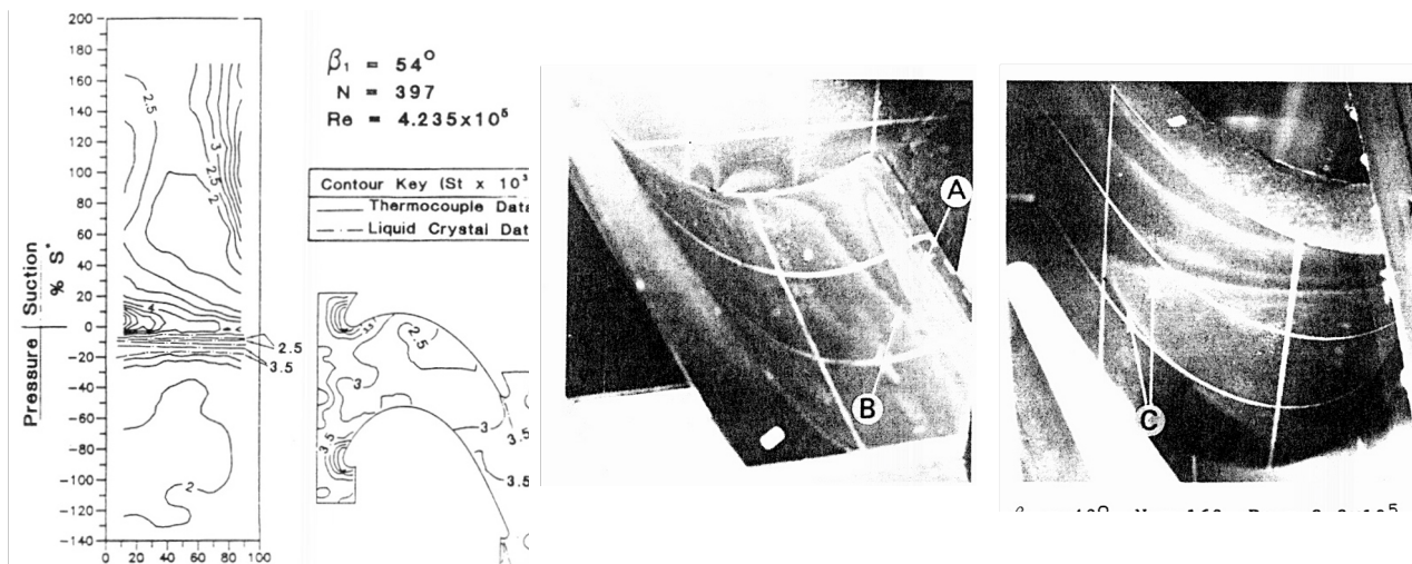
Figure 9. Stanton number measurements on the rotor surfaces of (LSRR) Blair et al. [1991]
