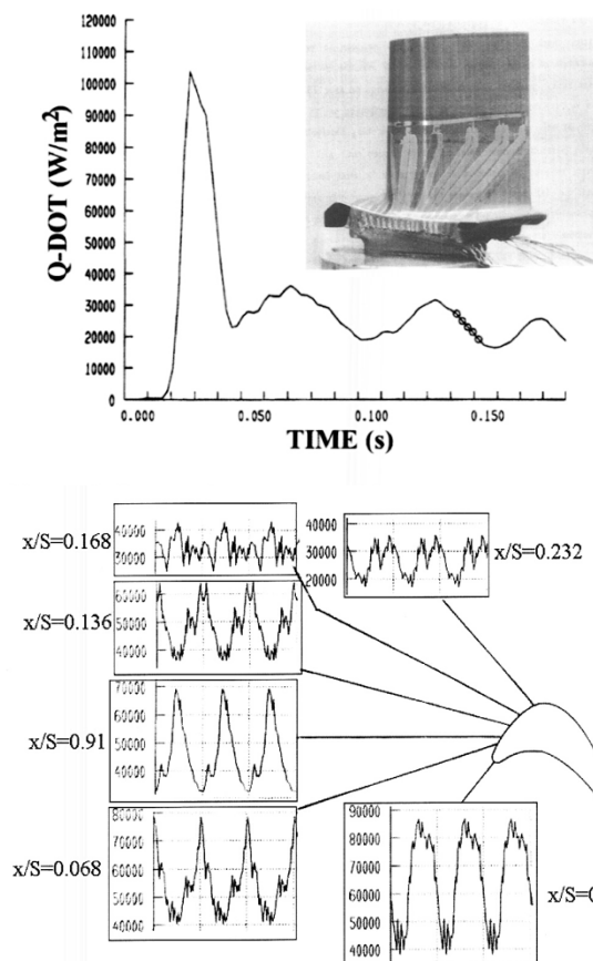
Figure 11. Unsteady heat flux sensors and heat flux measurements in turbine stage in the Oxford rotor facility ILPT, Allan et al., [2004]
