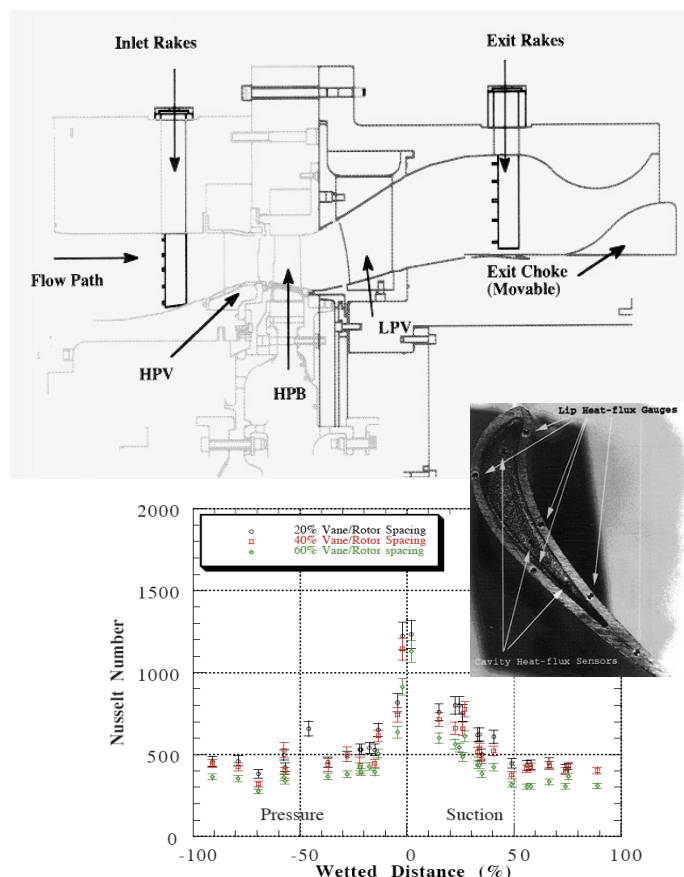
Figure 17. 1 and 1/2 stage turbine stage at Ohio State University, Haldeman et al. [2004] and Nusselt number distribution, Dunn and Haldeman [2000]
